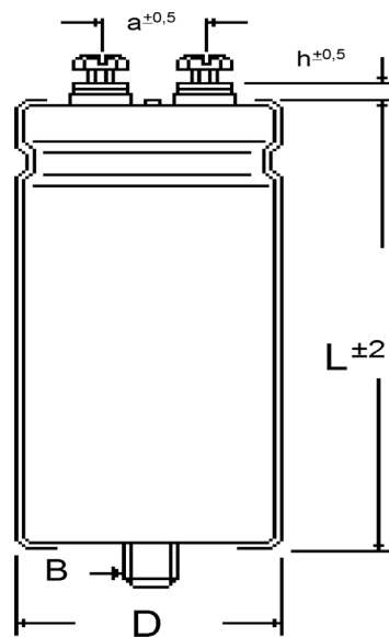
Fig2: GMXB for stud mounting
