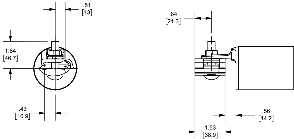
PARALLEL GROOVE
