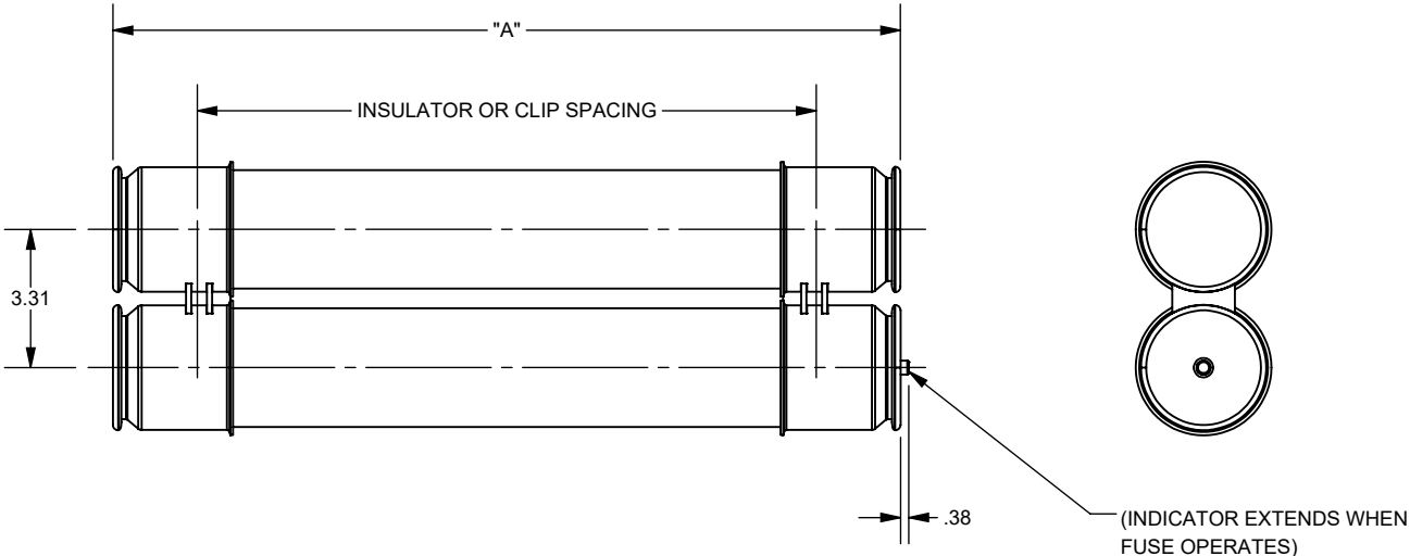
FIG 02 WITH DOUBLE FUSE OTHERWISE SAME AS FIG 01
