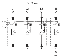
L 4+0 (4P)
