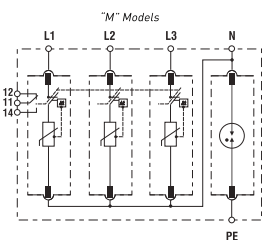
J 3+1 (4PG)
