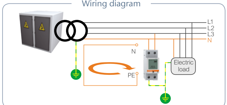
Wiring diagram
